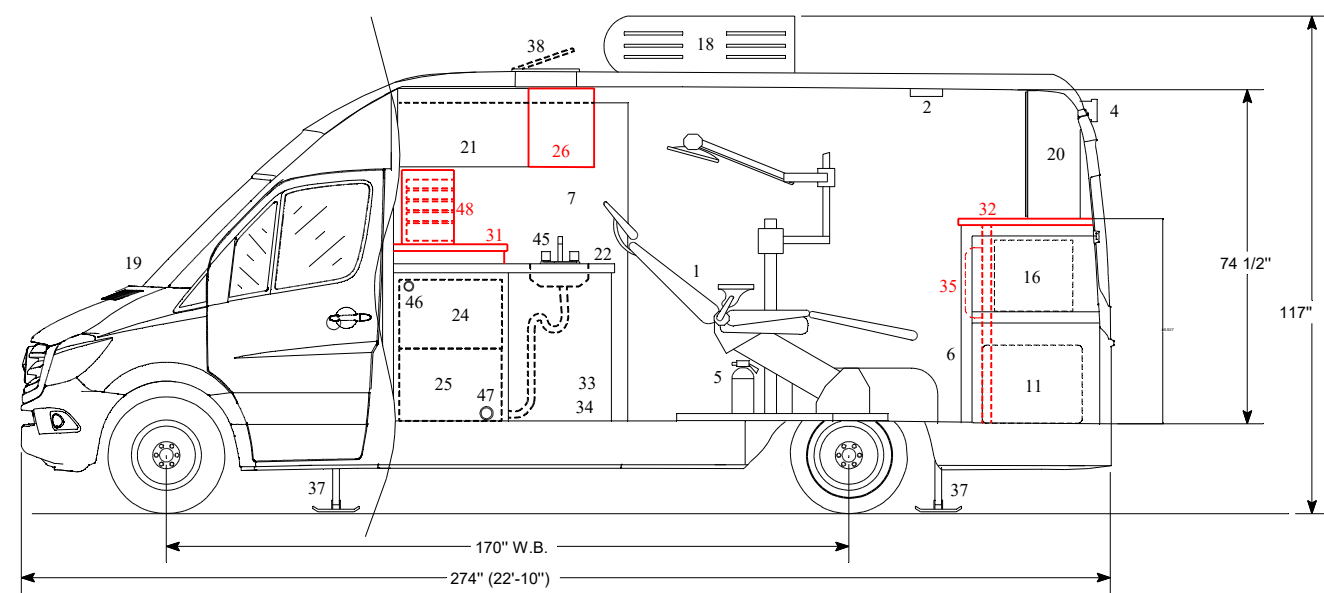
VIEW w/ STREET SIDE WALL REMOVED
