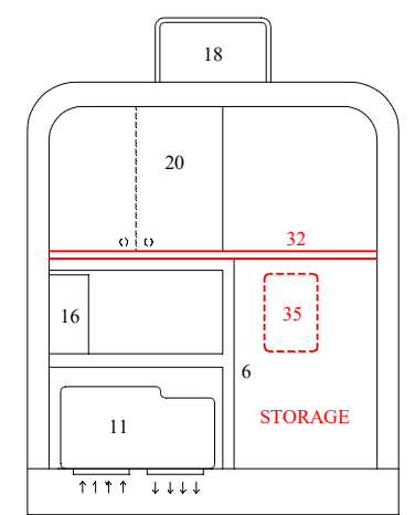
OUTSIDE VIEW w/ DOORS REMOVED LOOKING FORWARD.
